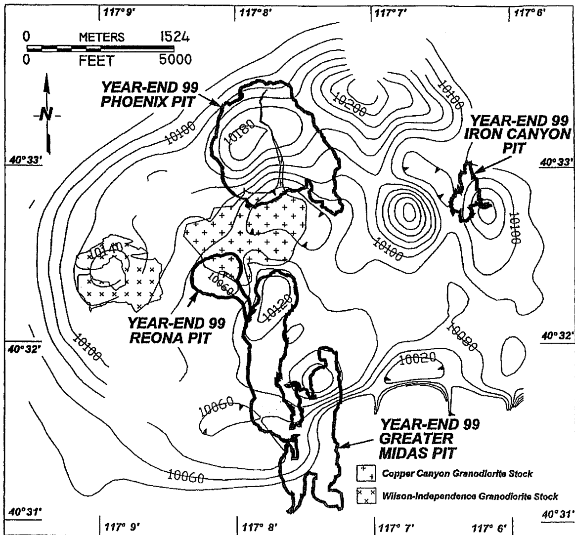
FIGURE 4. Aeromagnetic map of the Phoenix project area, Nevada showing year-end 1999 pits.
