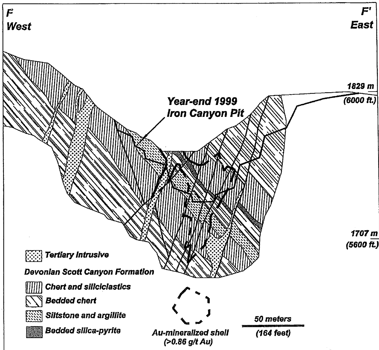
FIGURE 13. East-west cross-section F-F' through the Iron Canyon deposit showing geology and Au mineralization >0.86 g/t.
